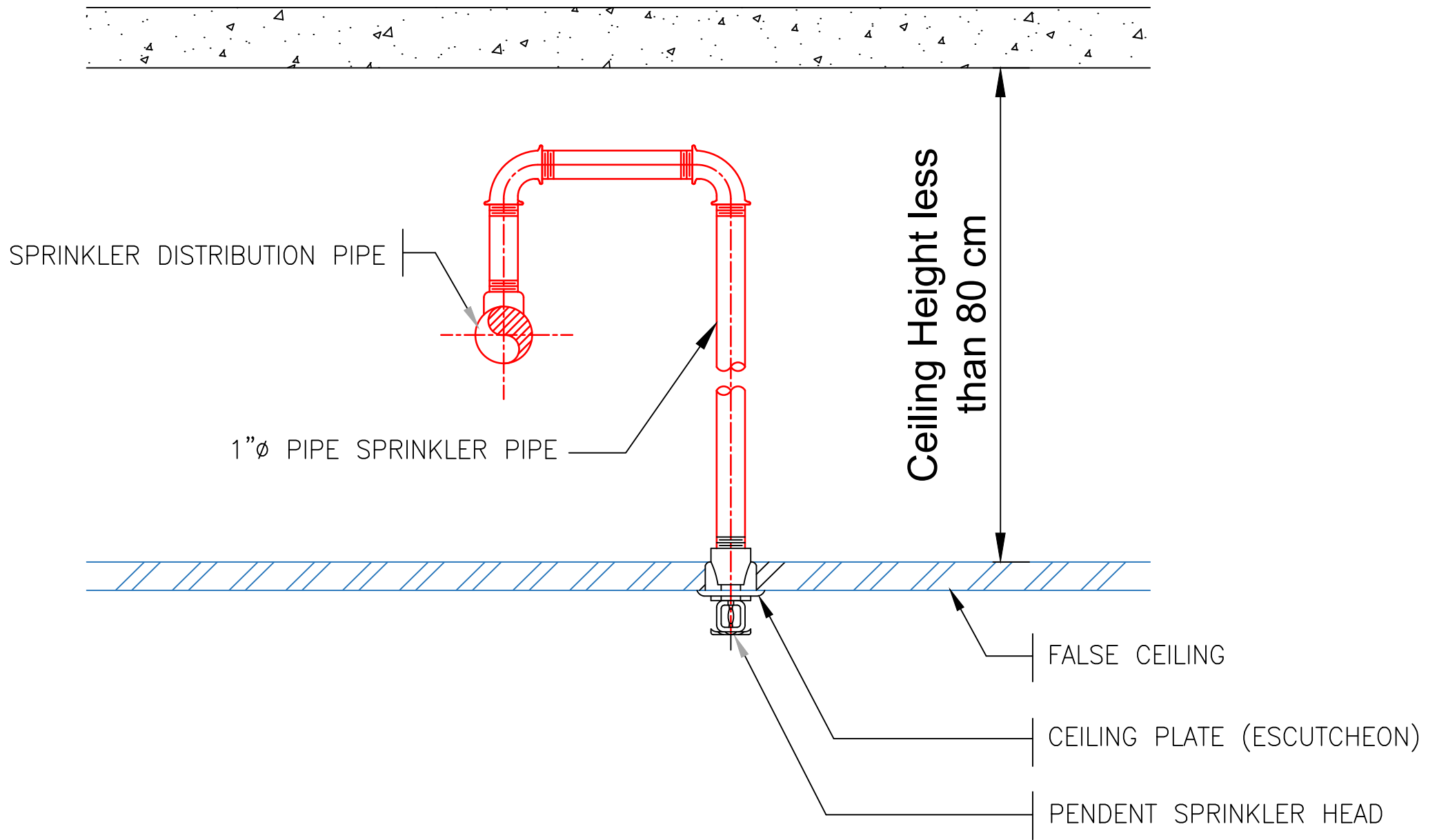
TYPICAL PENDENT SPRINKLER INSTALLATION (CEILING HEIGHT LESS THAN 80 CM)
